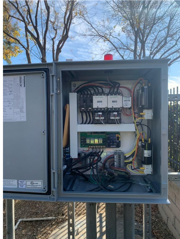
New storm water pump control panel for Heritage Farm Basin
